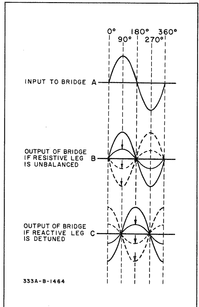
Figure 4-2. Bridge Waveforms
